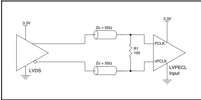
Figure 2A. PCLK/nPCLK Input Driven by a 3.3V LVDS Driver
