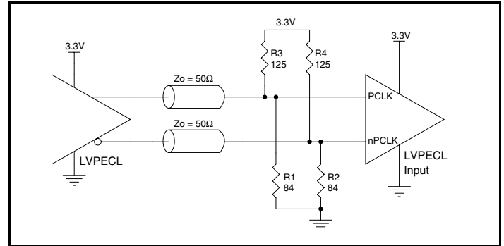
Figure 2B. PCLK/nPCLK Input Driven by a 3.3V LVPECL Driver
