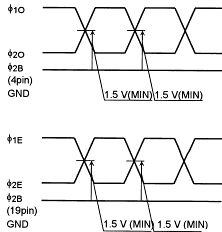
\phi 1 , \phi 2 CROSS POINT
