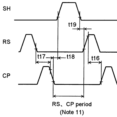
SH, RS, CP Timing
