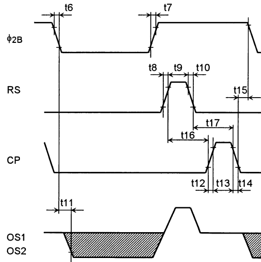
\phi 2 , RS, CP, OS Timing
