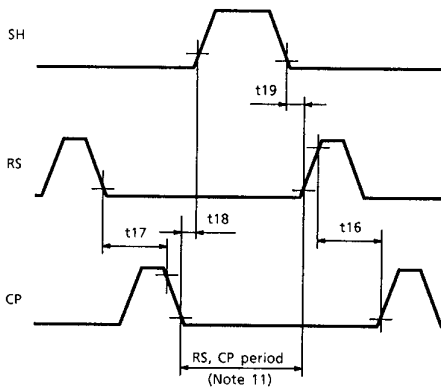
SH, RS, CP Timing
