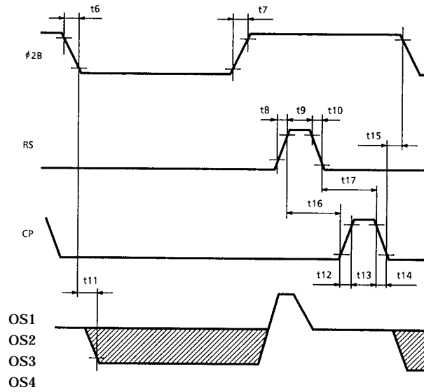
\phi 2 , RS, CP, OS Timing
