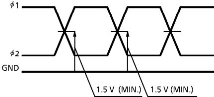
\phi 1 , \phi 2 CROSS POINT
