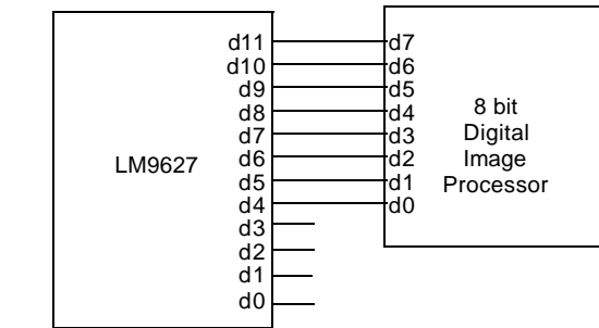
Figure 34. Example of connection to 10/8 bit systems
