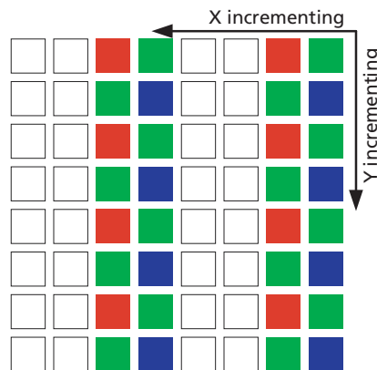
Figure 16: Pixel Readout (Column Skip 2X)
