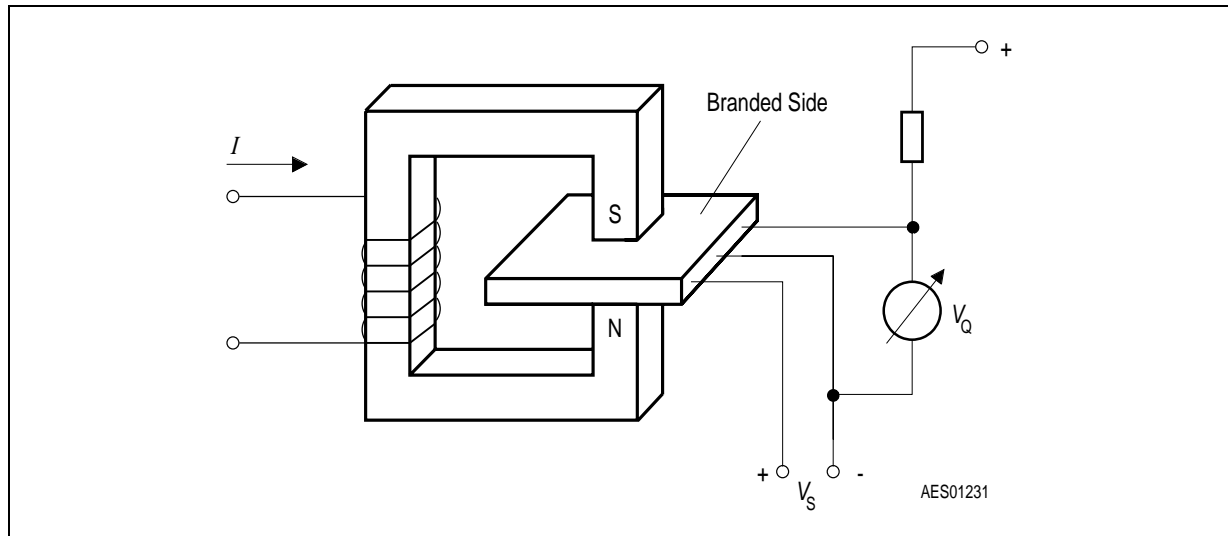
Figure 5 Sensor/Magnetic-Field Configuration
