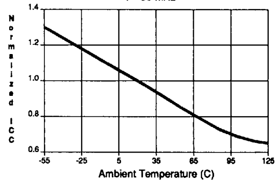
NORMALIZED ICC vs. AMBIENT TEMP. f = 30 MHz
