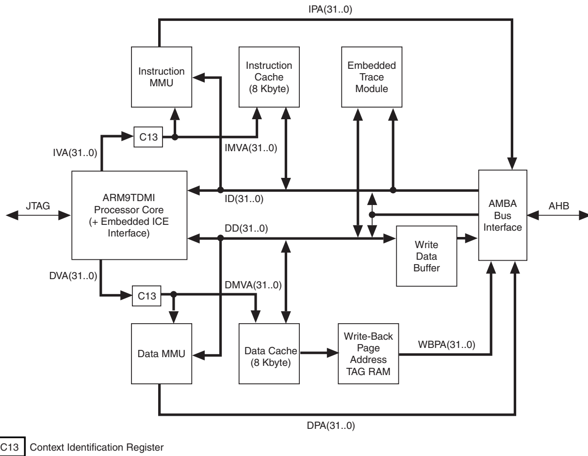
Figure 3. ARM922T Embedded Processor Internal Organization
