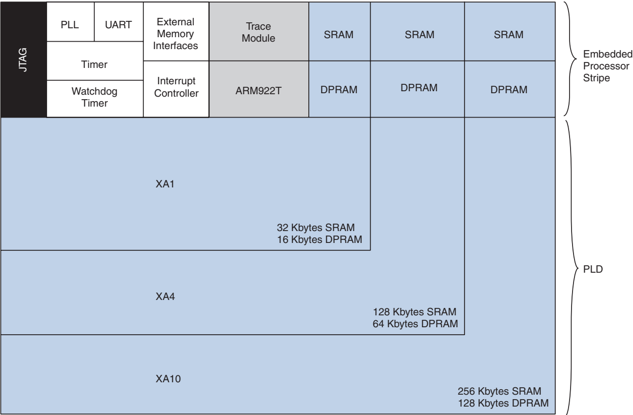
Figure 1. Excalibur Architecture
