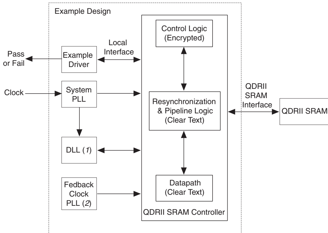
Figure 1–1. QDRII SRAM Controller System-Level Diagram
