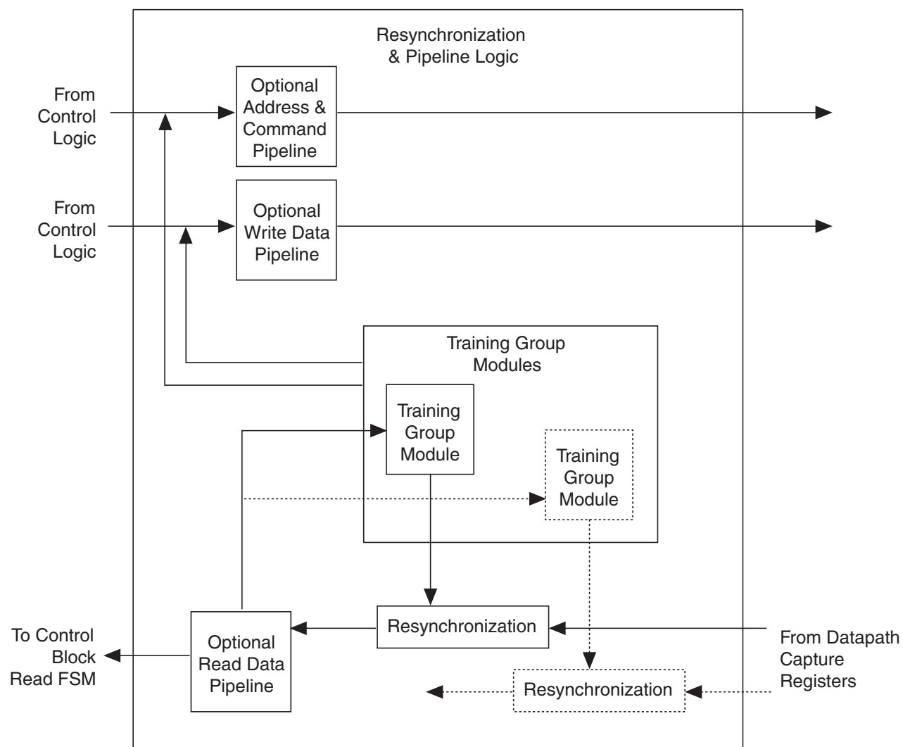
Figure 3–3. Resynchronization & Pipeline Logic Block Diagram
