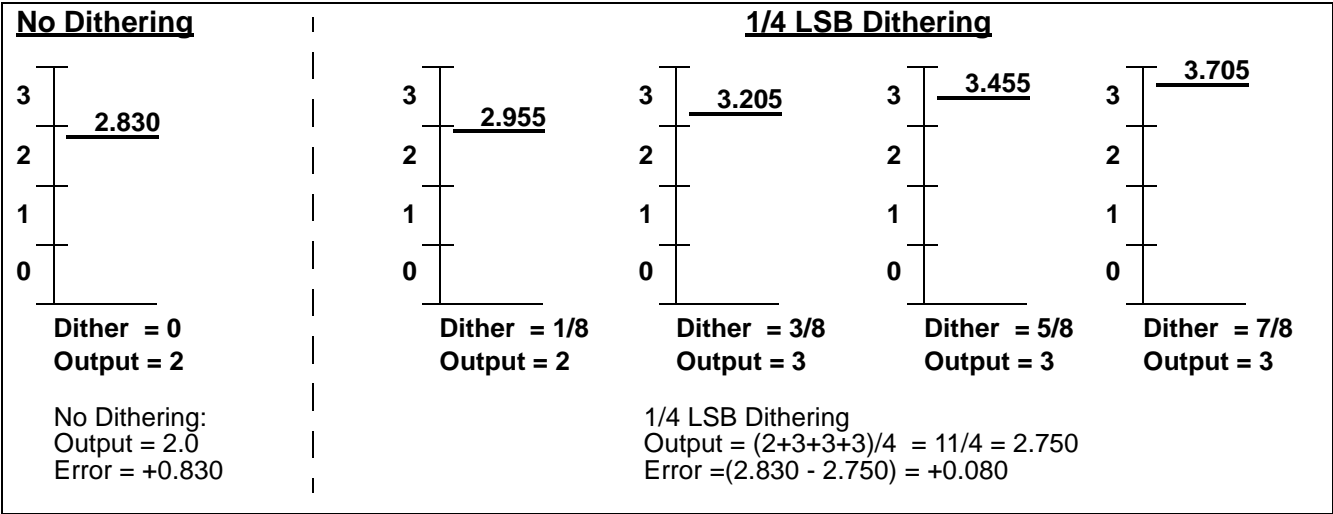
Figure 14-10. Dithering
