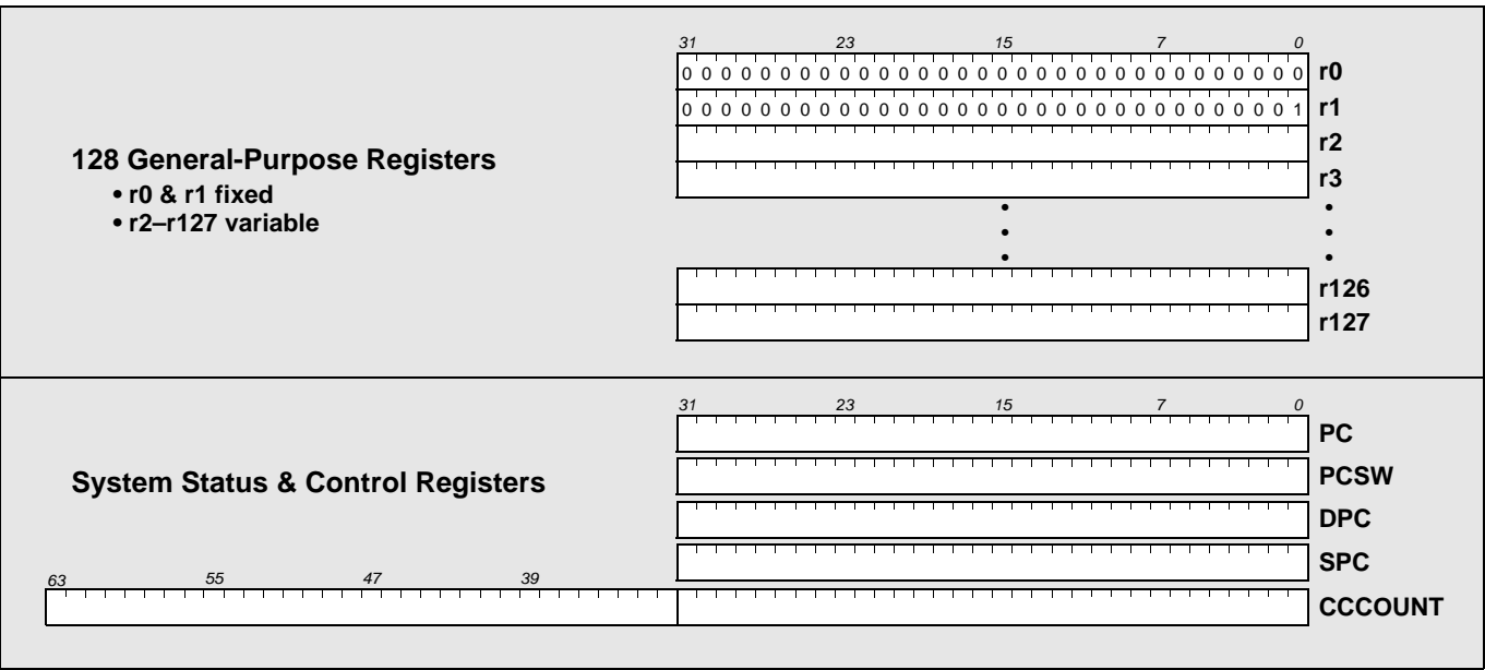
Figure 3-1. PNX1300 registers.
