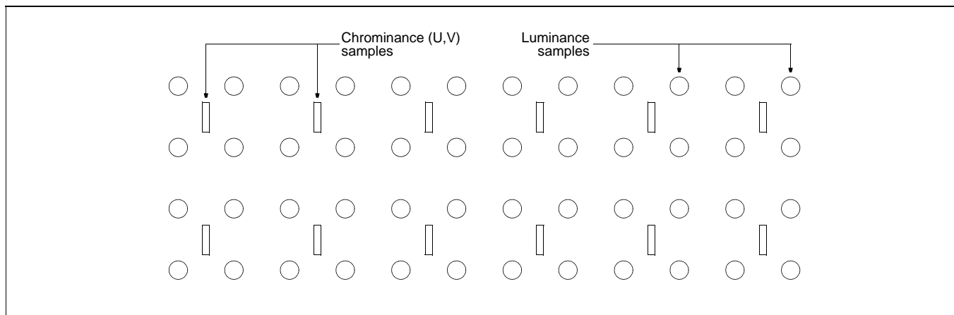
Figure 7-21. YUV 4:2:0 format.
