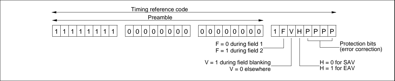
Figure 6-8. Format of CCIR656 SAV and EAV timing reference codes.
