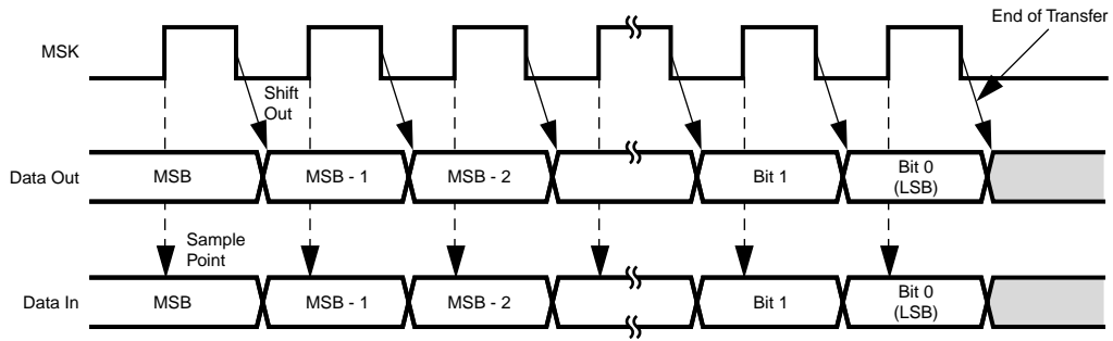
Figure 75. Normal Mode (SCIDL = 0)
