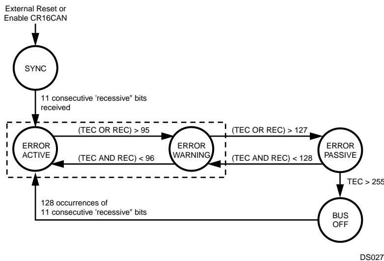
Figure 33. Bus States
