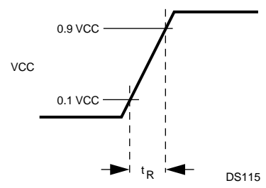
Figure 103. Power-On Reset
