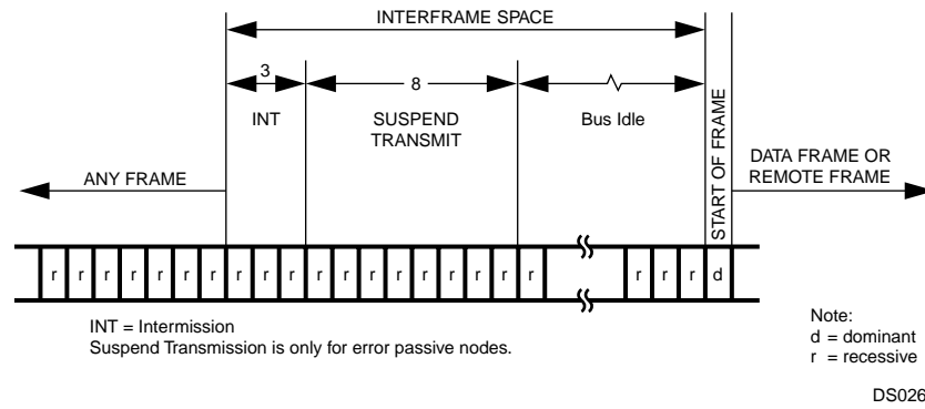
Figure 32. Interframe Space
