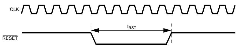
Figure 102. Non-Power-On Reset
