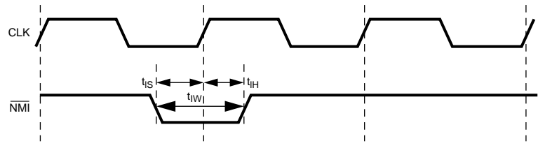
Figure 101. \overline{\text{NMI}} Signal Timing
