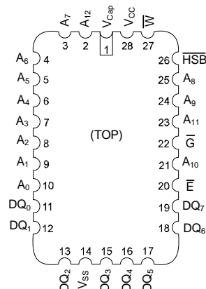
28-pin LCC
