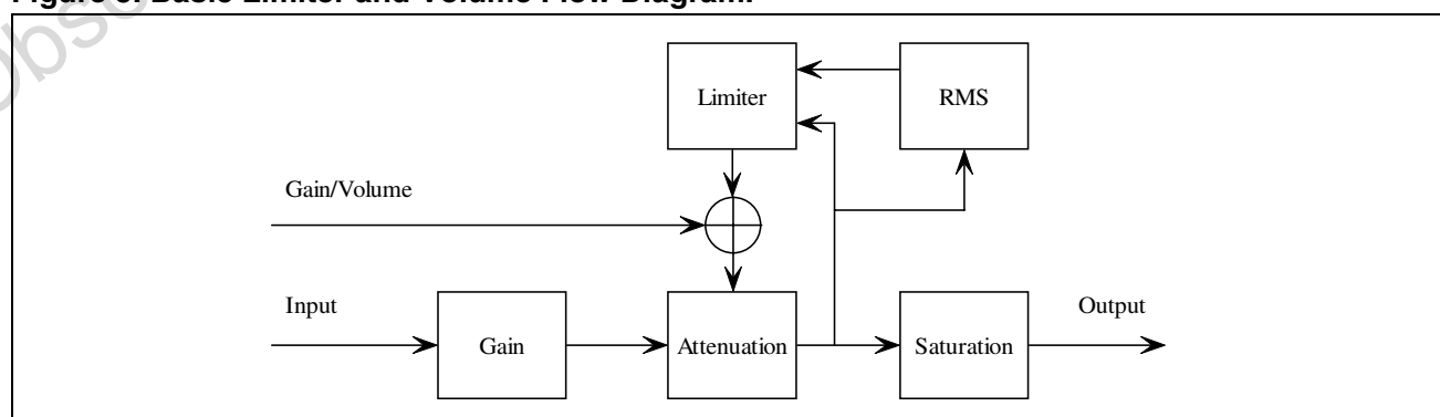
Figure 5. Basic Limiter and Volume Flow Diagram.
