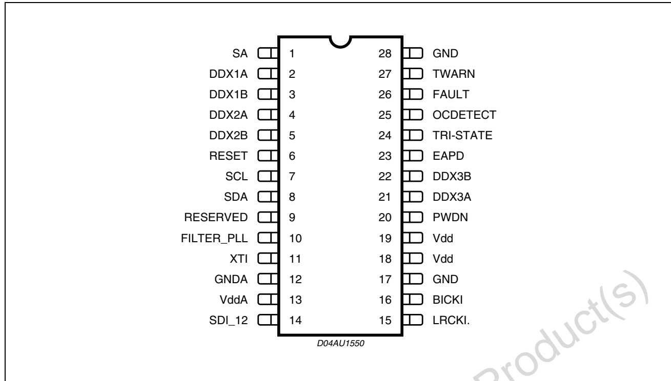
Figure 2. PIN CONNECTION (Top view)
