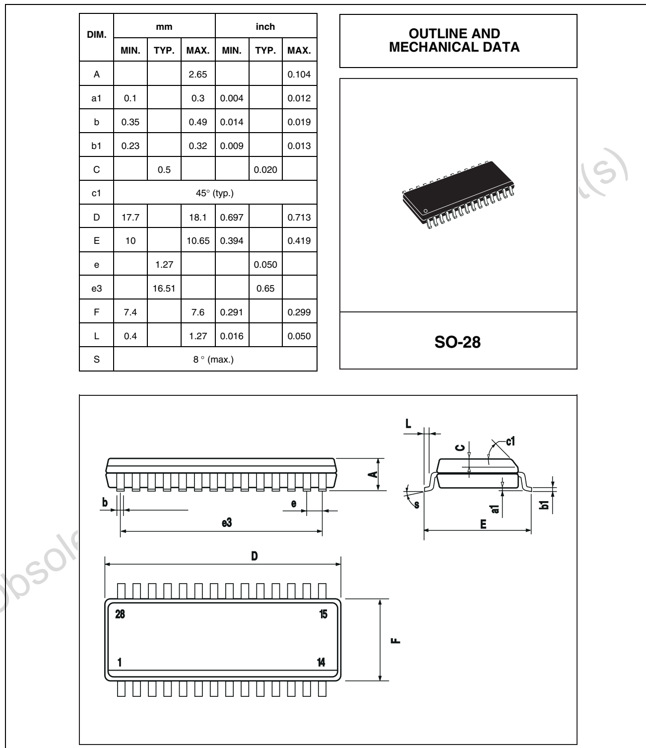
Figure 6. SO28 Mechanical Data & Package Dimensions
