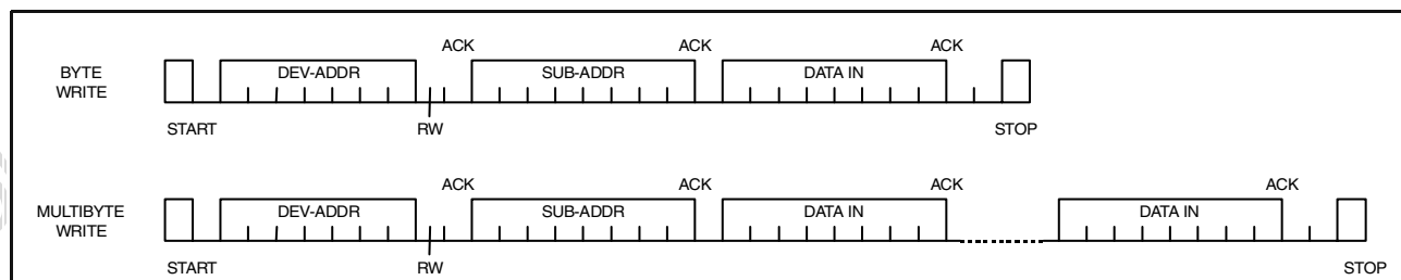
Figure 3. Write Mode Sequence
