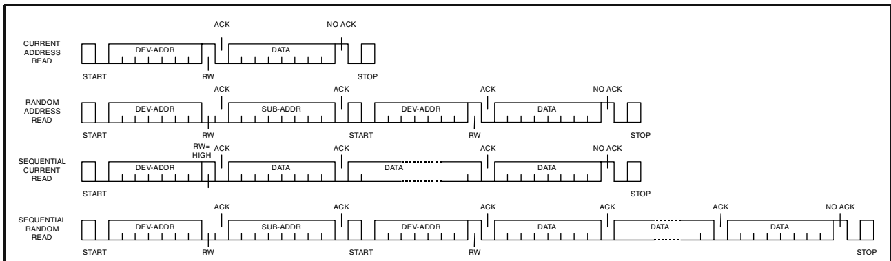
Figure 4. Read Mode Sequence
