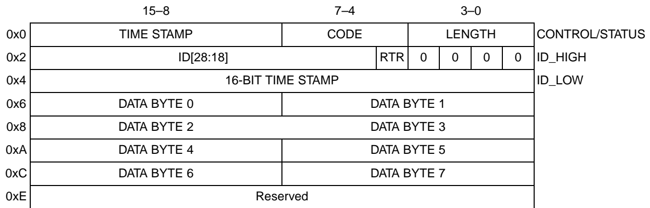
Figure 25-4. Standard ID Message Buffer Structure
