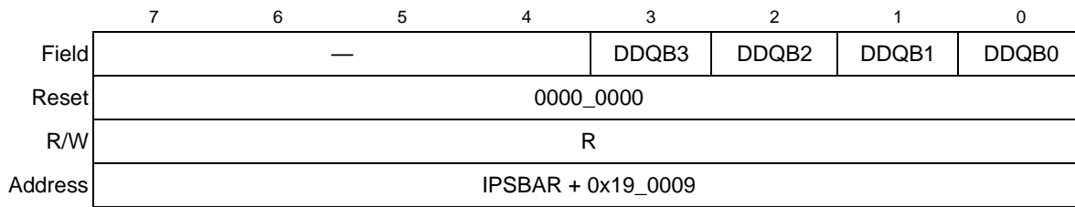
Figure 28-7. Port QB Data Direction Register (DDRQB)
