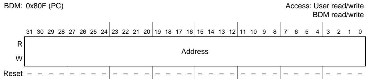
Figure 2-6. Program Counter Register (PC)
