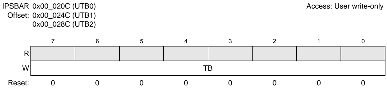
Figure 23-9. UART Transmit Buffer (UTB n )
