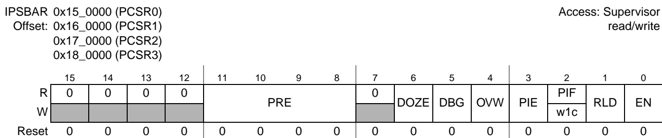
Figure 19-2. PCSR n Register
