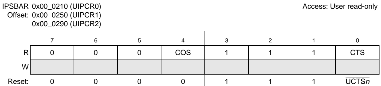
Figure 23-10. UART Input Port Changed Registers (UIPCR n )
