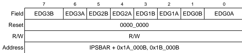
Figure 20-11. GPT Control Register 2 (GPTCTL2)
