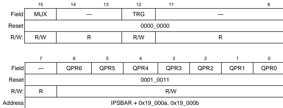
Figure 28-8. QADC Control Register 0 (QACR0)
