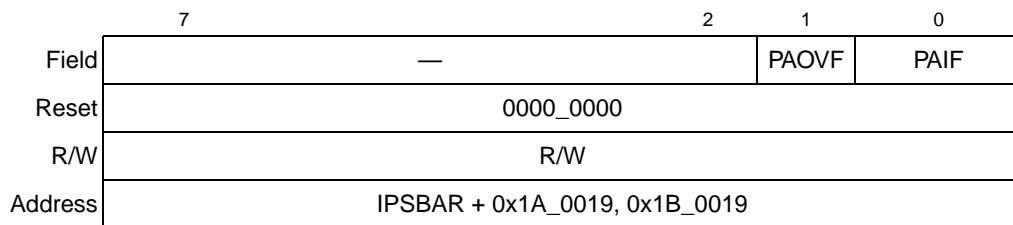
Figure 20-18. Pulse Accumulator Flag Register (GTPAFLG)
