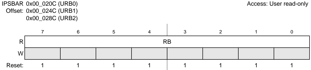
Figure 23-8. UART Receive Buffer (URB n )
