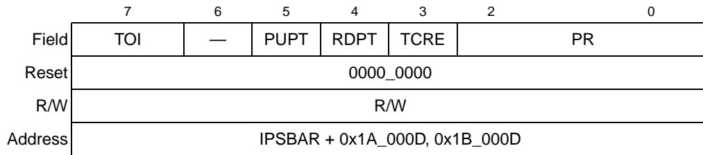
Figure 20-13. GPT System Control Register 2 (GPTSCR2)
