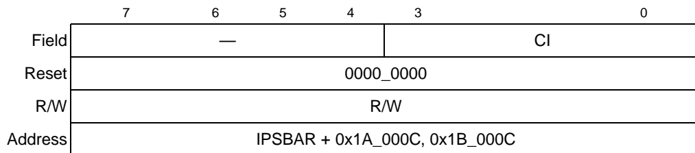
Figure 20-12. GPT Interrupt Enable Register (GPTIE)
