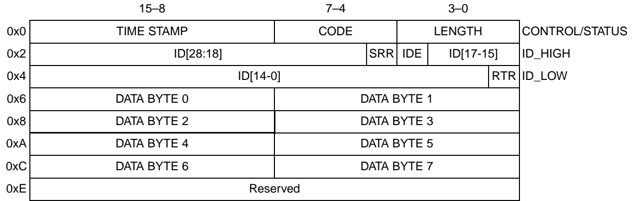
Figure 25-3. Extended ID Message Buffer Structure
