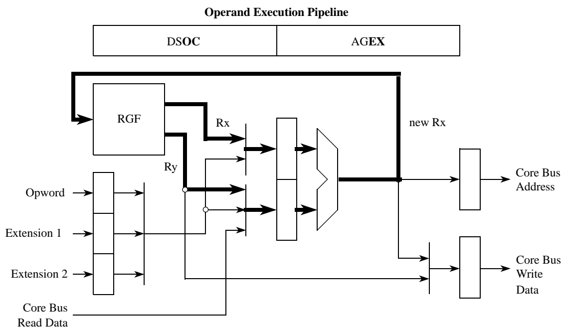
Figure 2-11. V2 OEP Register-to-Register
