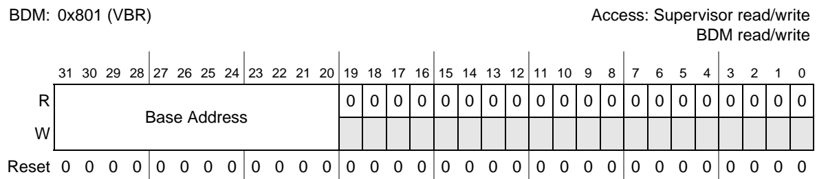
Figure 2-7. Vector Base Register (VBR)
