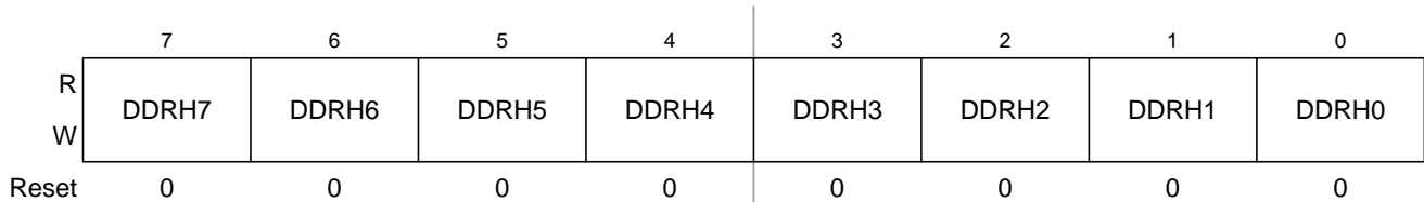
Figure 23-50. Port H Data Direction Register (DDRH)
