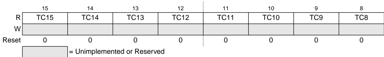
Figure 7-63. Timer Input Capture Holding Register 3 High (TC3H)
