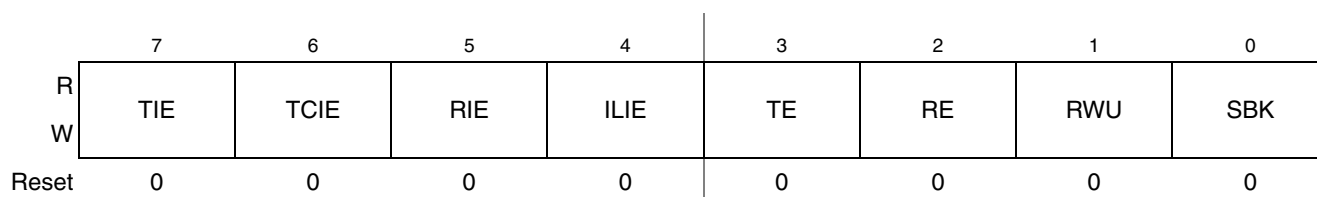
Figure 14-8. SCI Control Register 2 (SCIC2)
