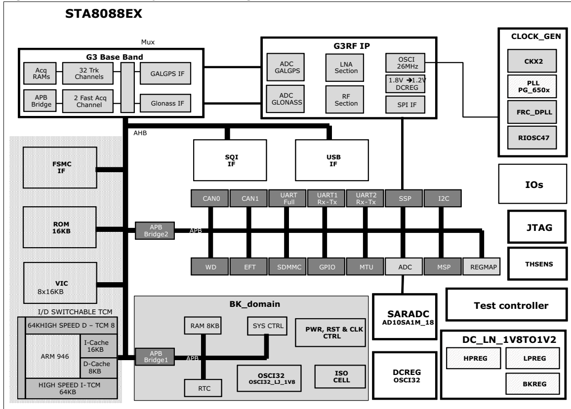
Figure 1. STA8088EX system block diagram
