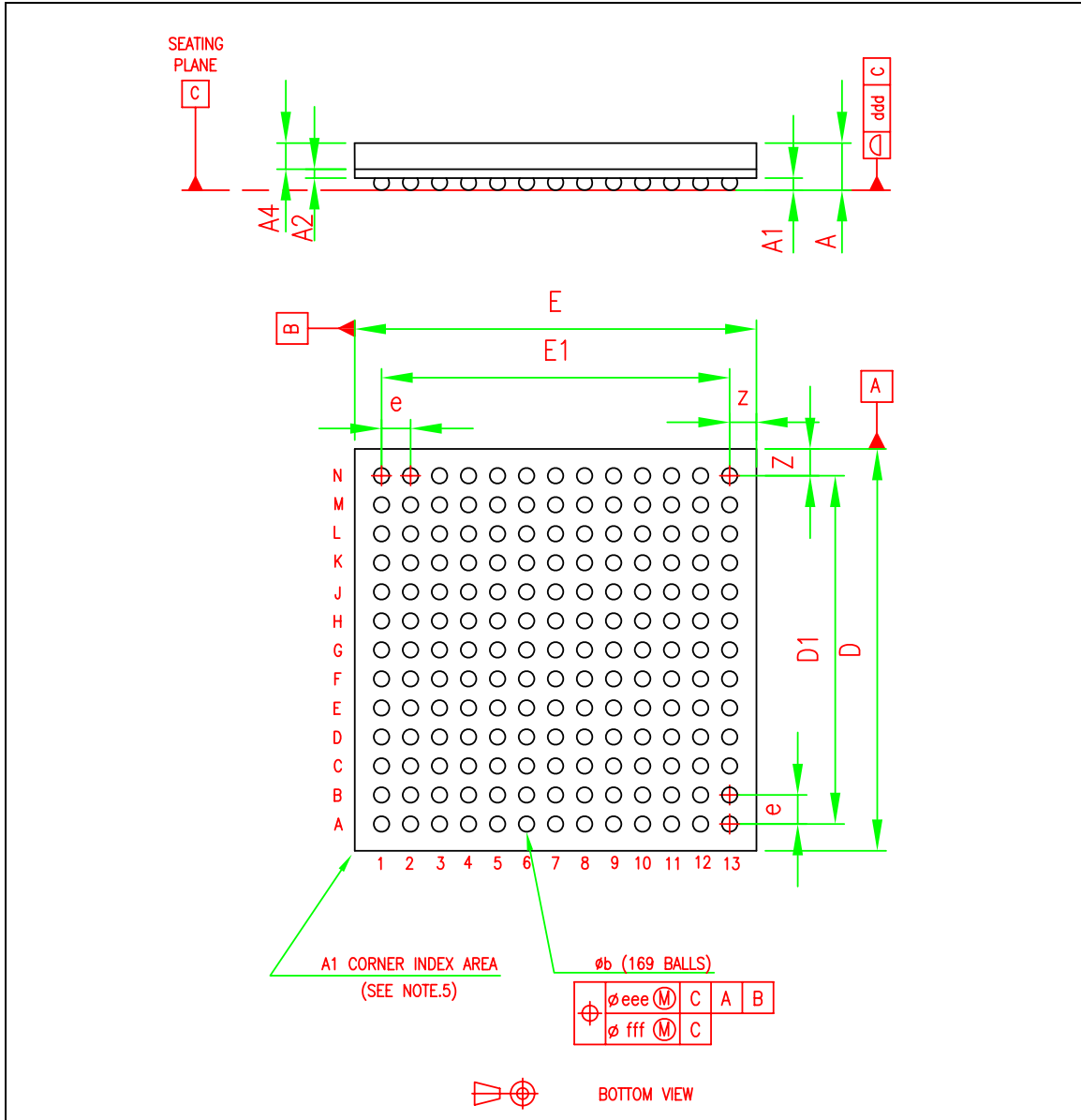
Figure 2. TFBGA169 package dimension
