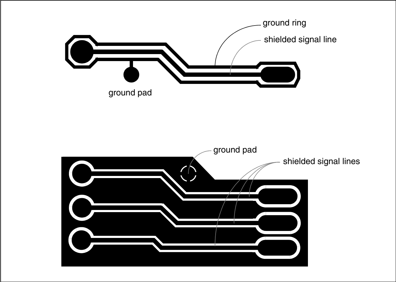
Figure 6-20. Shielding signals
