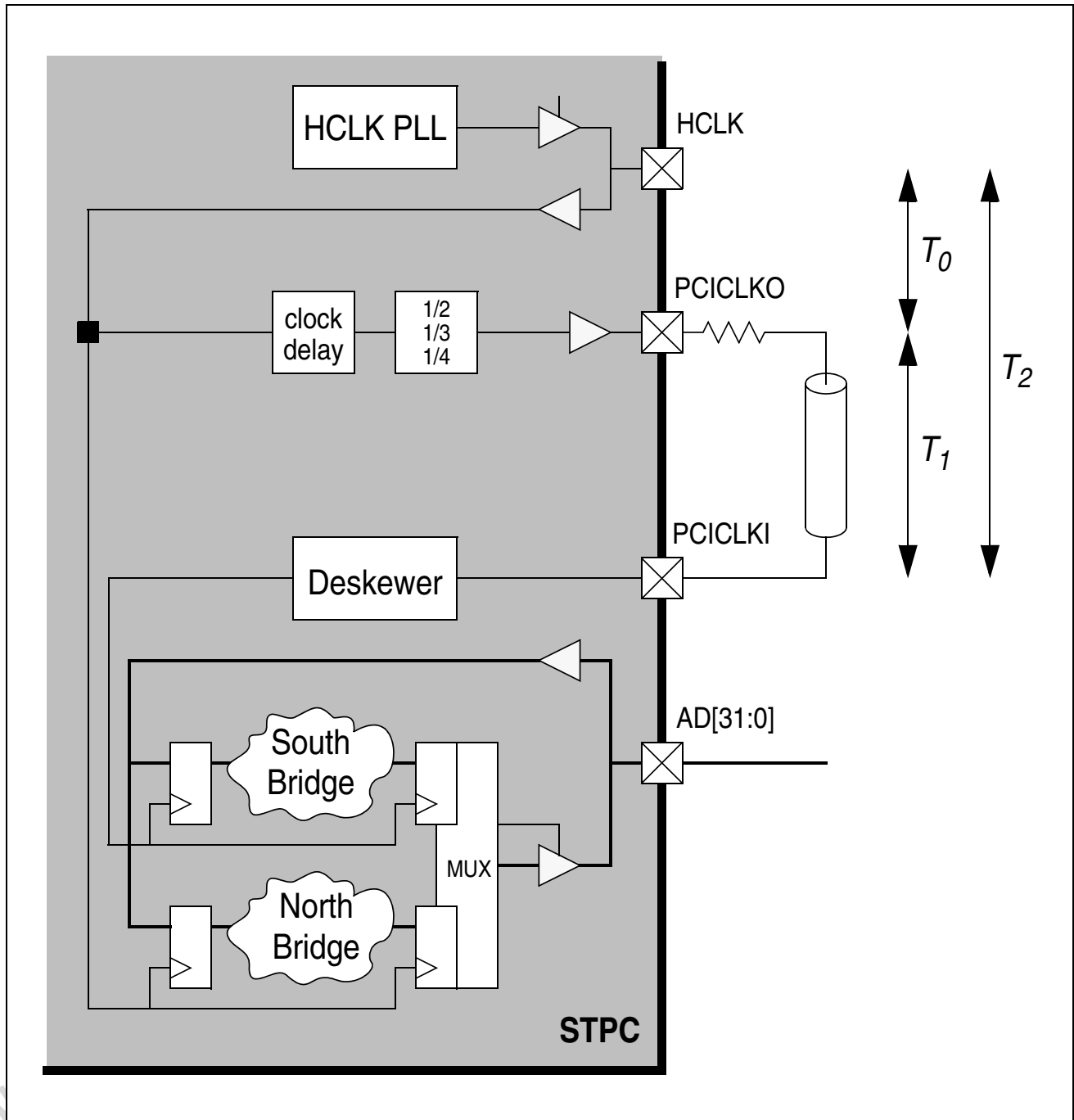
Figure 6-28. Clock Scheme
