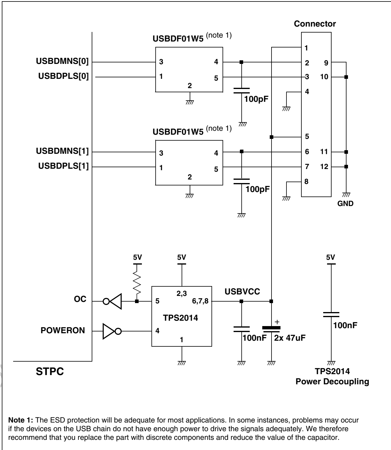
Figure 6-16. Typical USB implementation
