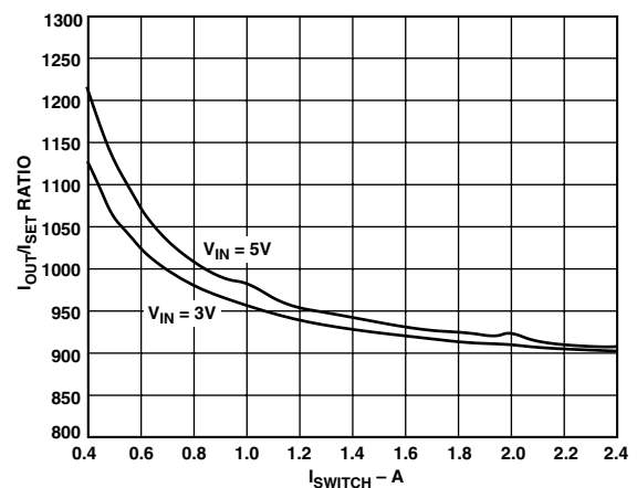
TPC 6. I_{\text{OUT}}/I_{\text{SET}} Ratio vs. Switch Current
