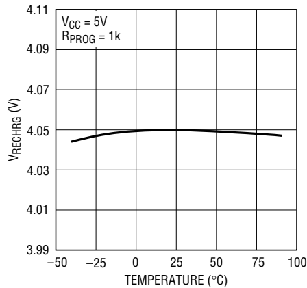
Recharge Voltage Threshold vs Temperature
