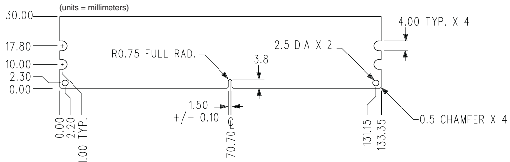
Figure 1: KVR400D2S8R3/1G 240-Pin DIMM
