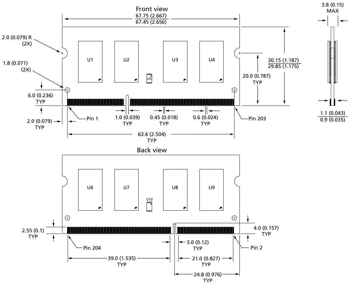
Figure 5: 204-Pin DDR3 SODIMM
