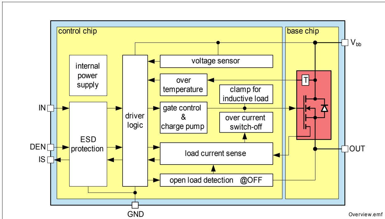
Figure 1 Block Diagram
