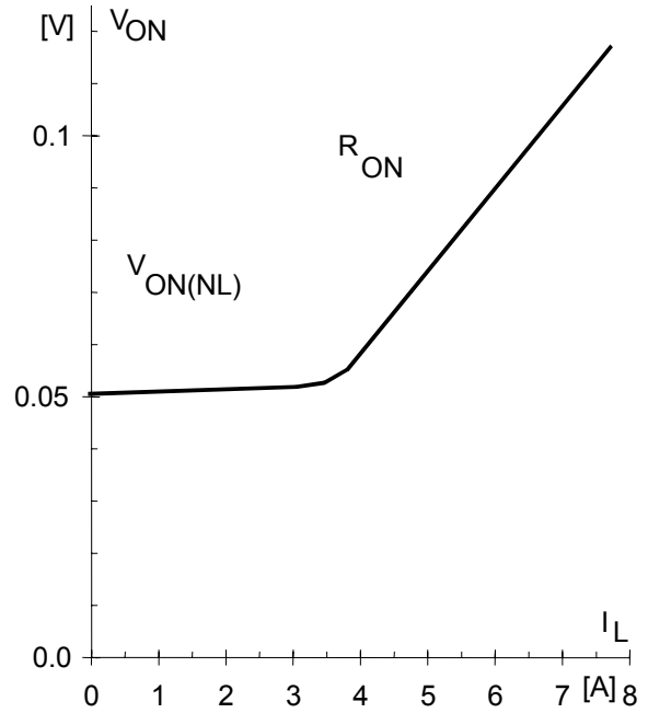
Figure 7a: Output voltage drop versus load current:
