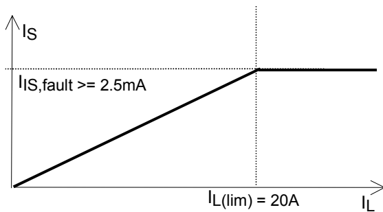
Figure 1b: typical behaviour of sense output:
