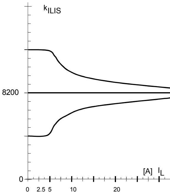
Figure 6b: Current sense ratio 12) :
