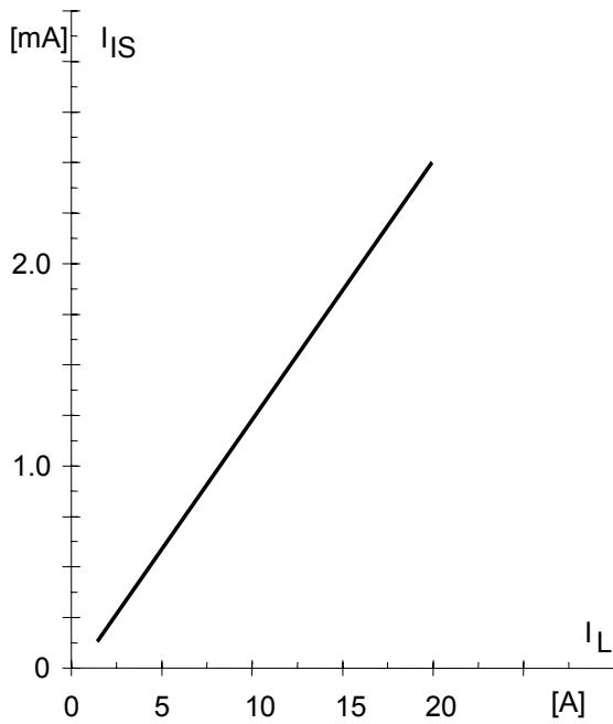
Figure 6b: Current sense ratio 12) :
