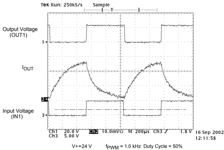
Figure 13. Output Voltage and Current vs. Input Voltage at V+ = 24 V, PMW Frequency of 1.0 kHz, and Duty Cycle of 50%
