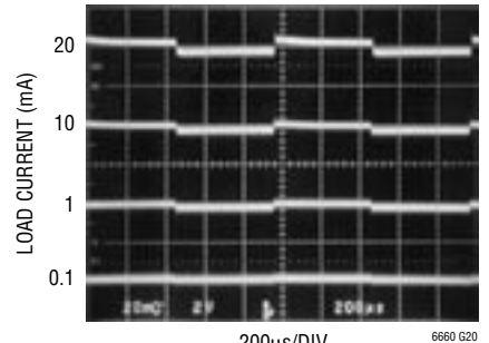
10V Transient Response
