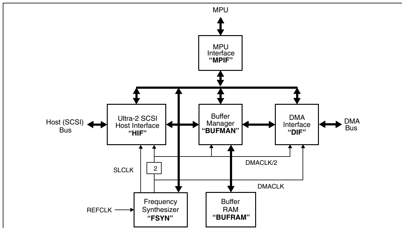
Figure 2. AIC-43C97C Block Diagram
