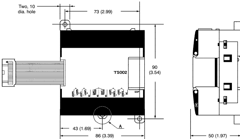
CPM1A-TS□□□ Temperature Sensor Input Modules
