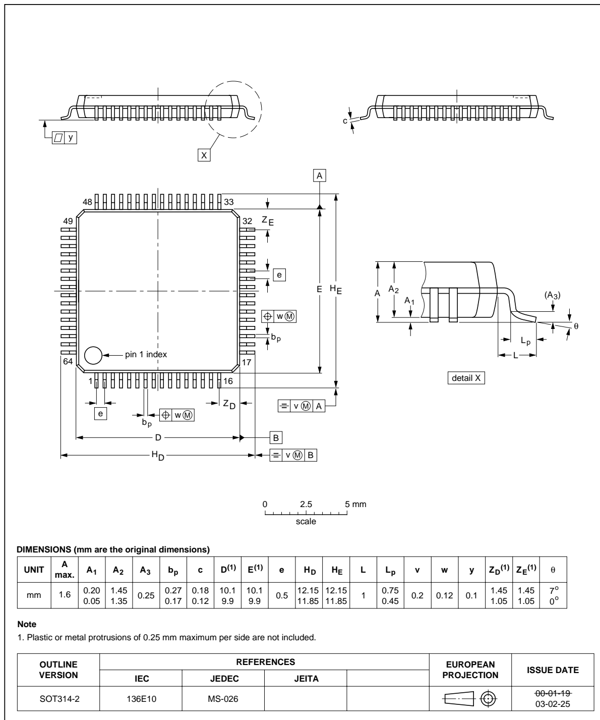
Fig 43. LQFP64 (SOT314-2) package outline.
