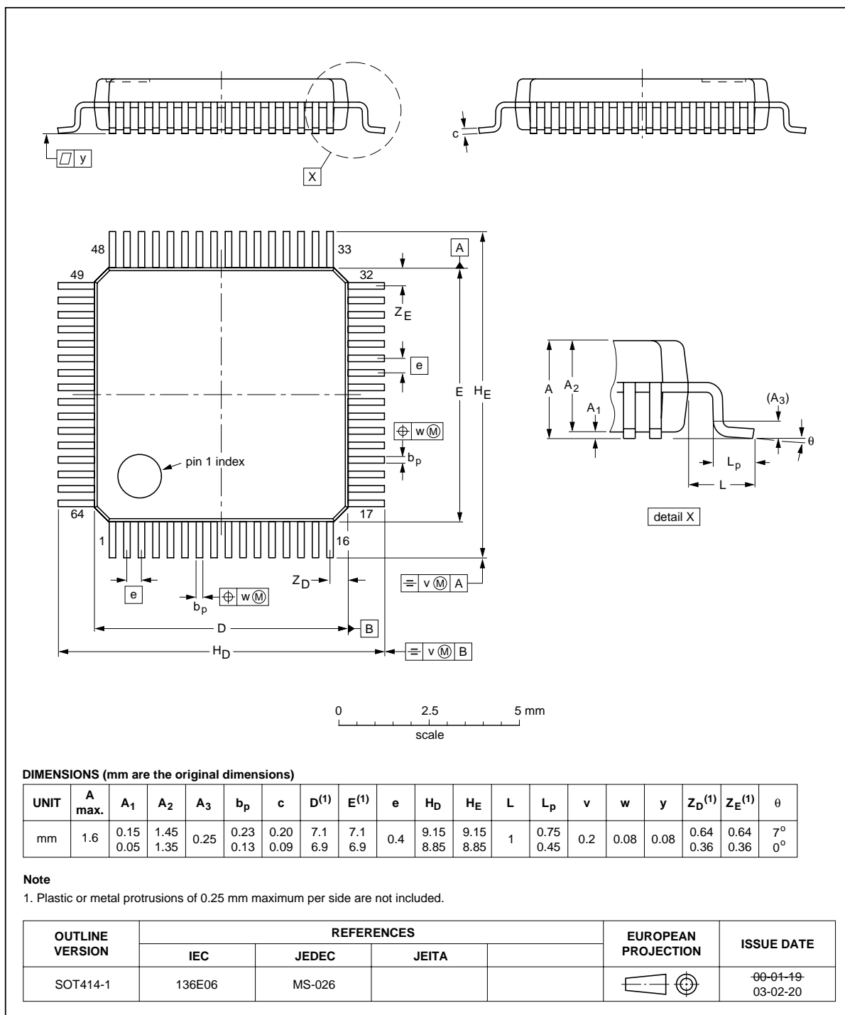
Fig 44. LQFP64 (SOT414-1) package outline.
