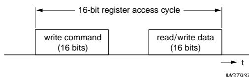
Fig 6. 16-bit register access cycle.
