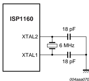
Fig 31. Oscillator circuit with external crystal.
