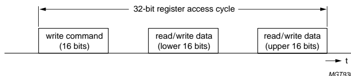
Fig 7. 32-bit register access cycle.
