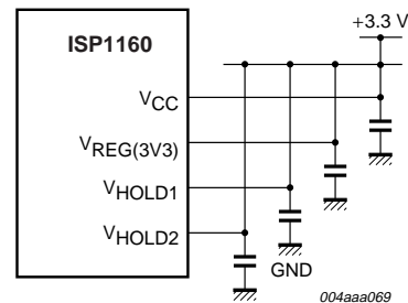
Fig 30. Using a 3.3 V supply.
