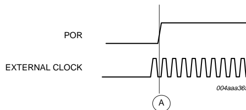
Fig 34. Clock with respect to the external POR.
