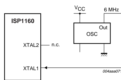
Fig 32. Oscillator circuit using external oscillator.
