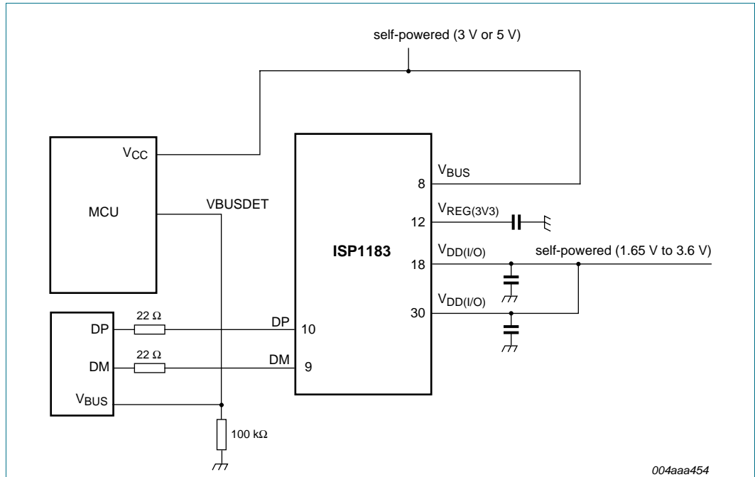
Fig 25. V BUS connected to the microprocessor
