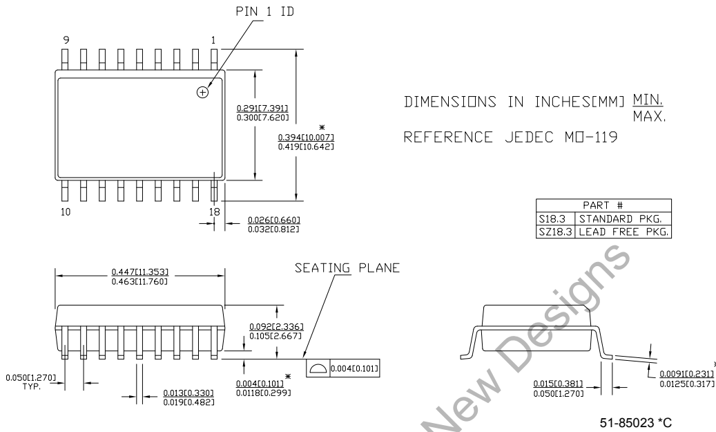
Figure 37. 18-Pin (300-Mil) Molded SOIC S1
