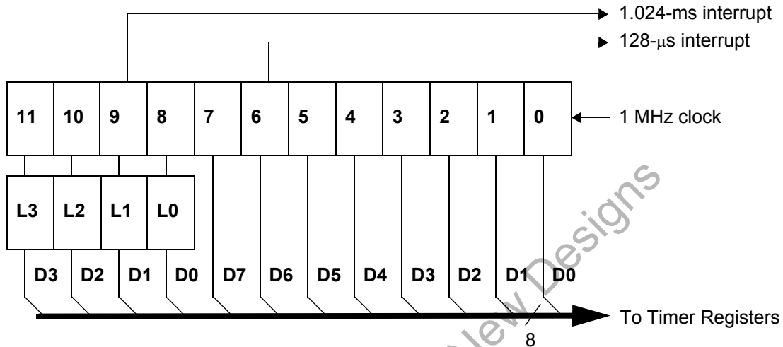
Figure 21. Timer Block Diagram
