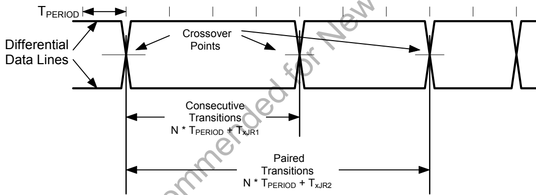
Figure 35. Differential Data Jitter
