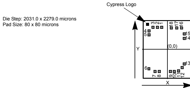
Figure 39. Die Form DIE FORM
