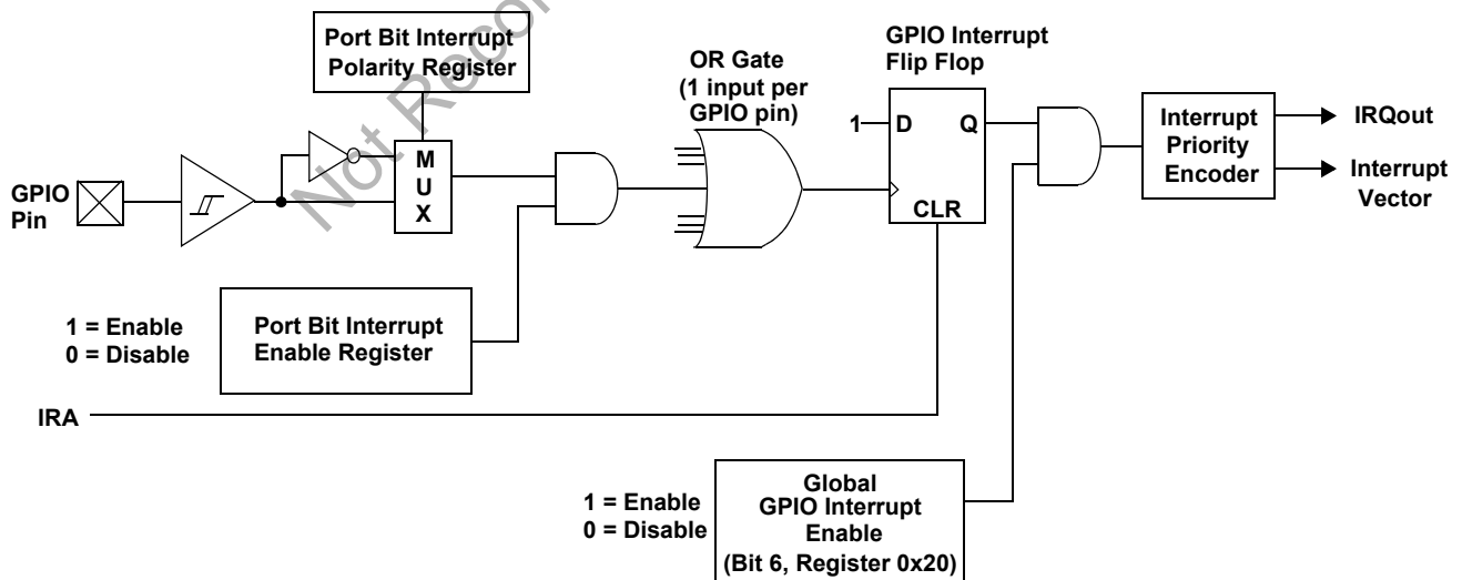
Figure 30. GPIO Interrupt Diagram
