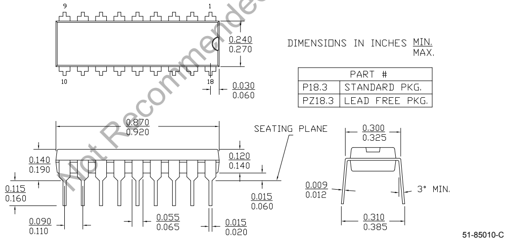
Figure 38. 18-Pin (300-Mil) Molded DIP P3
