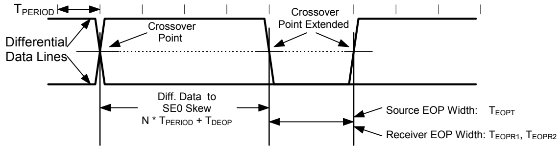
Figure 34. Differential to EOP Transition Skew and EOP Width
