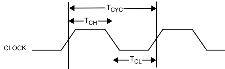
Figure 31. Clock Timing
