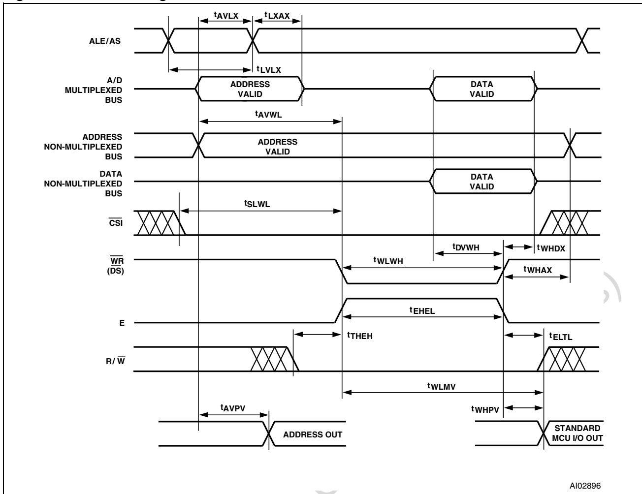
Figure 41. WRITE Timing
