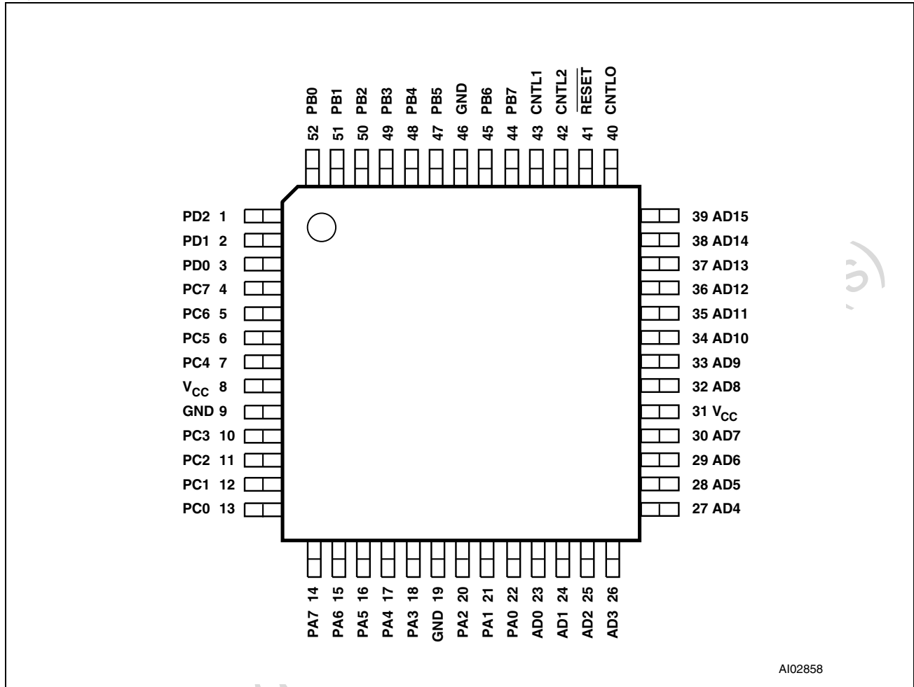
Figure 46. PQFP52 Connections
