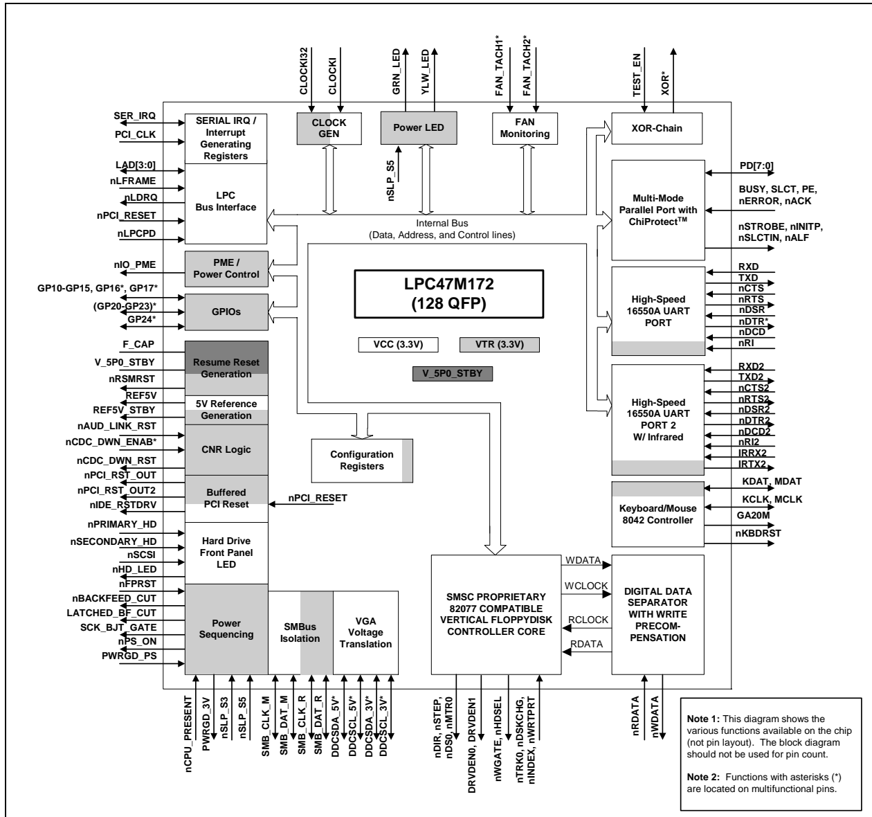
Figure 1 - LPC47M172 Block Diagram
