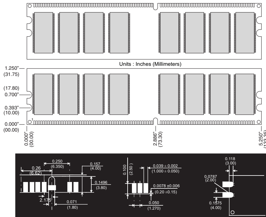
Figure 1: KVR400X64C25/512 184-Pin DDR SDRAM Module
