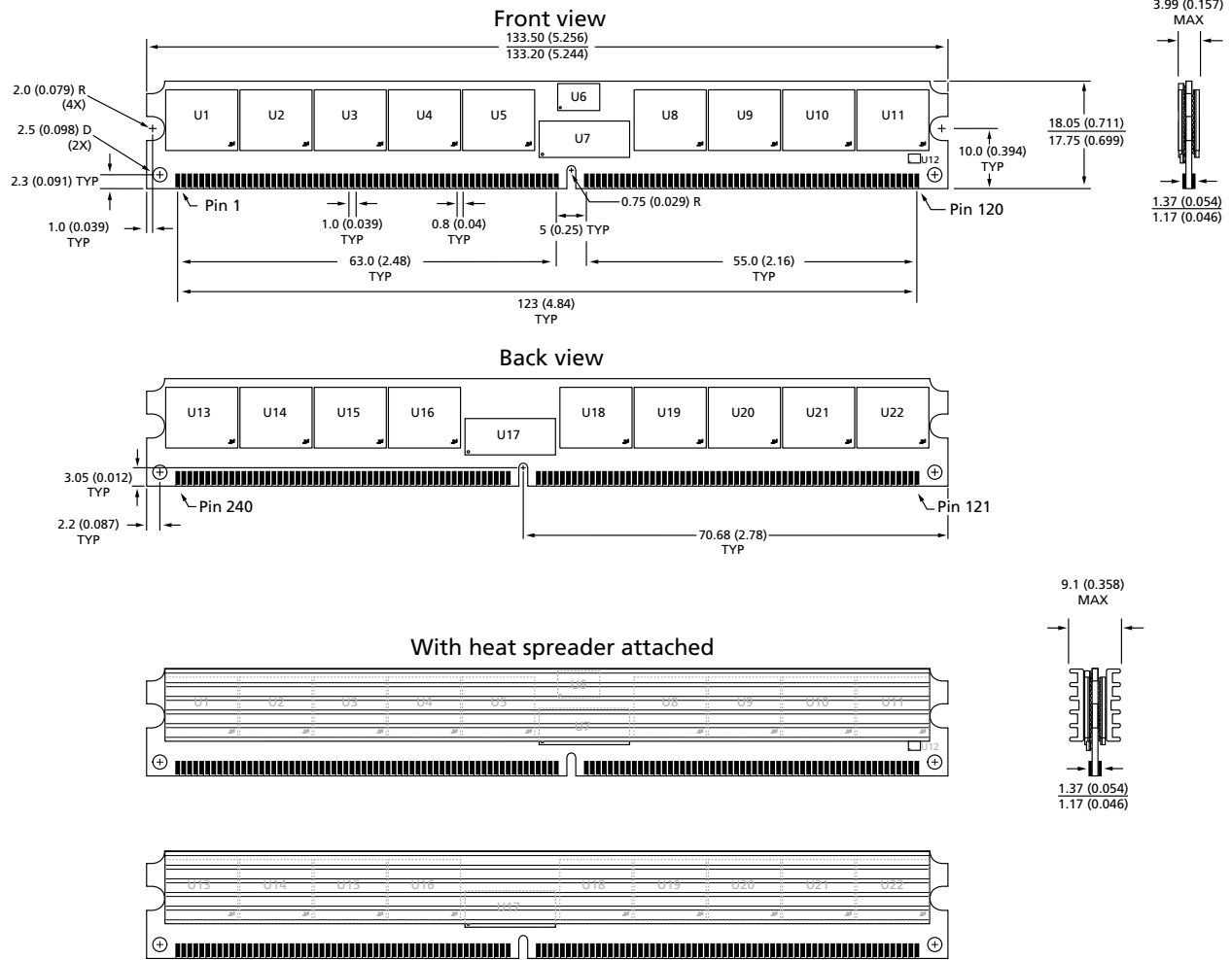
Figure 3: 240-Pin DDR2 VLP RDIMM
