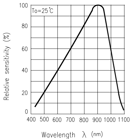
Fig.3 Spectral Sensitivity
