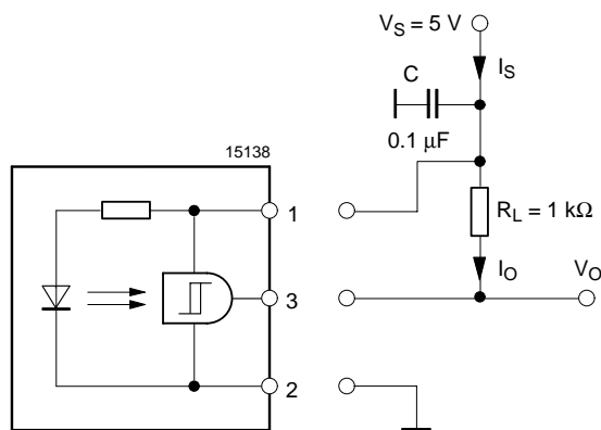
Figure 1. Test circuit and pin connection
