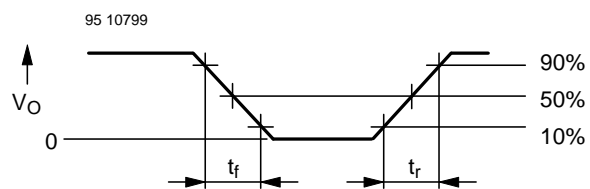
Figure 2. Pulse diagram
