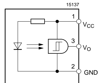
Pin connection
