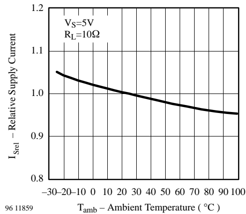
Figure 5. Relative Supply Current vs. Ambient Temperature
