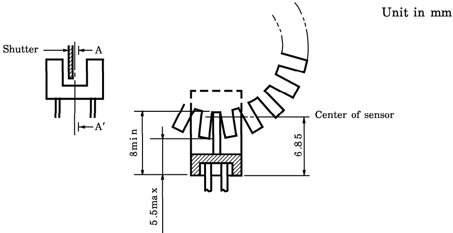
Cross section between A and A'
