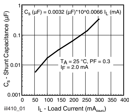
Fig. 1 - Shunt Capacitance vs. Load Current
