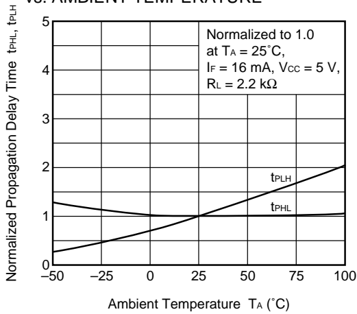
NORMALIZED PROPAGATION DELAY TIME vs. AMBIENT TEMPERATURE
