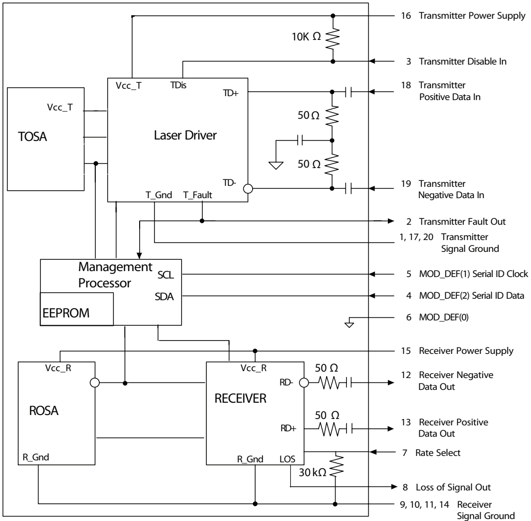
Figure 1 Block diagram
