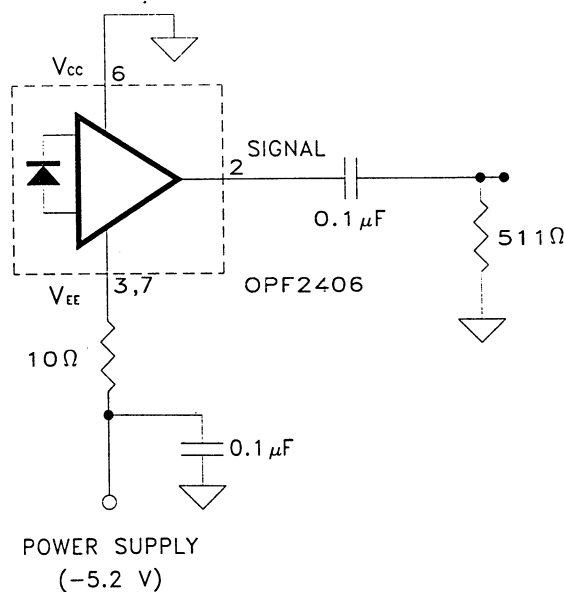
Recommended AC Coupled Receiver Circuit
