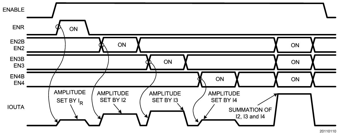
Functional Timing Diagram
