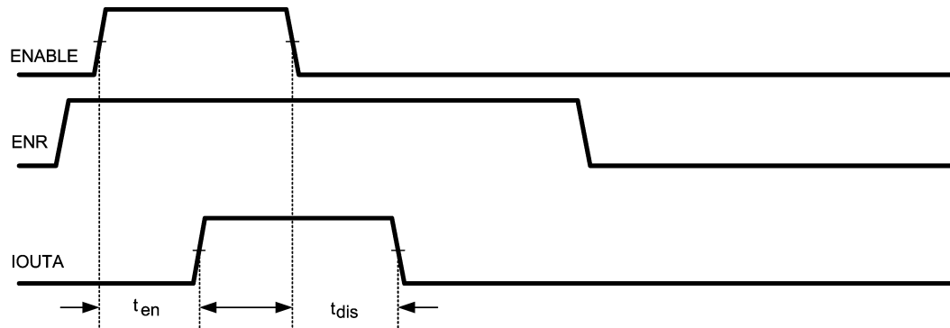
Enable Timing
