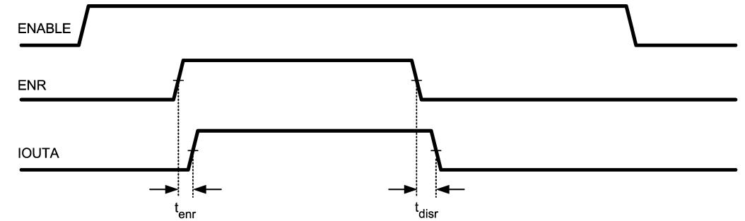
Read Timing
