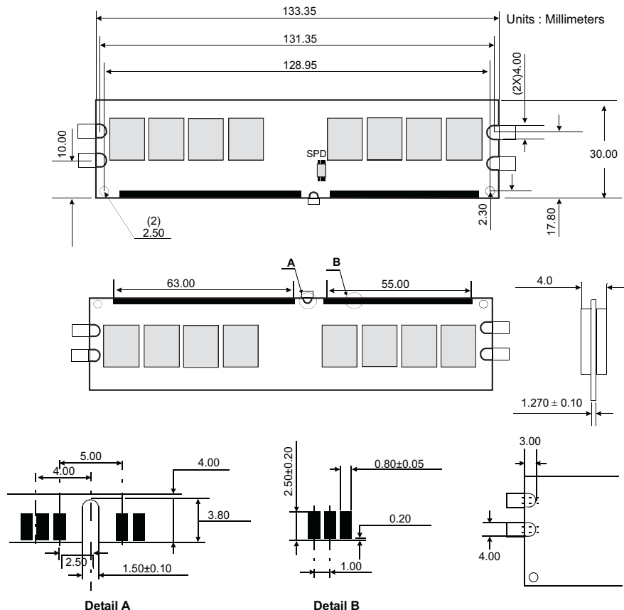
Figure 1: KVR667D2N5/2G 240-Pin DIMM
