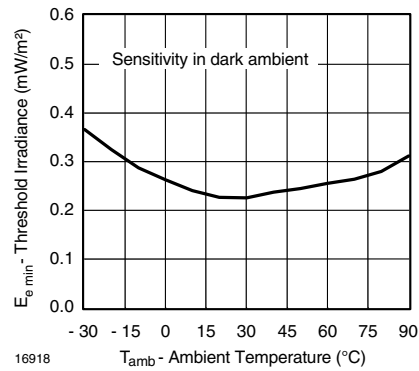
Figure 10. Sensitivity vs. Ambient Temperature
