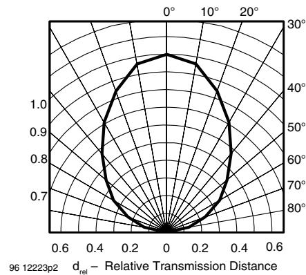
Figure 12. Directivity
