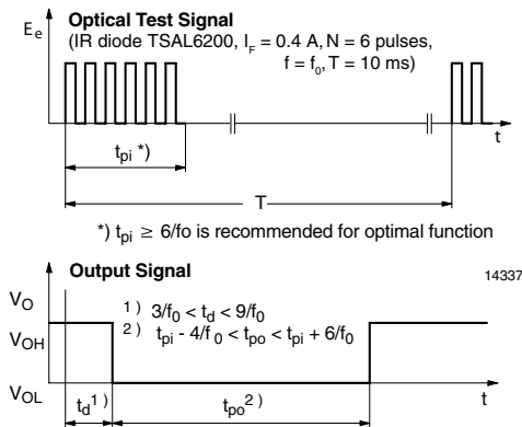
Figure 1. Output Function
