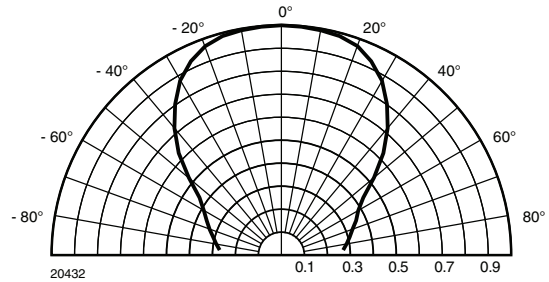
Fig. 12 - Directivity
