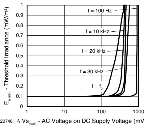
Fig. 7 - Sensitivity vs. Supply Voltage Disturbances
