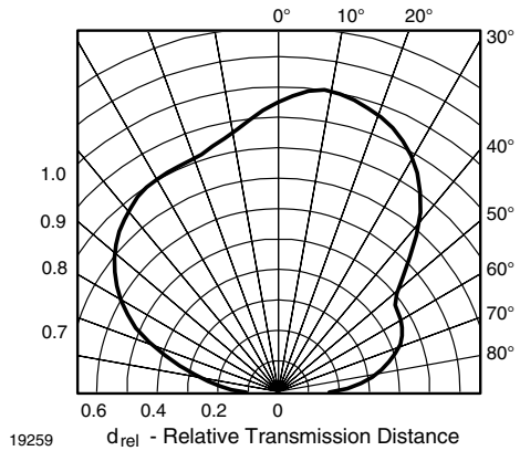
19259 d_{rel} - Relative Transmission Distance Fig. 13 - Vertical Directivity
